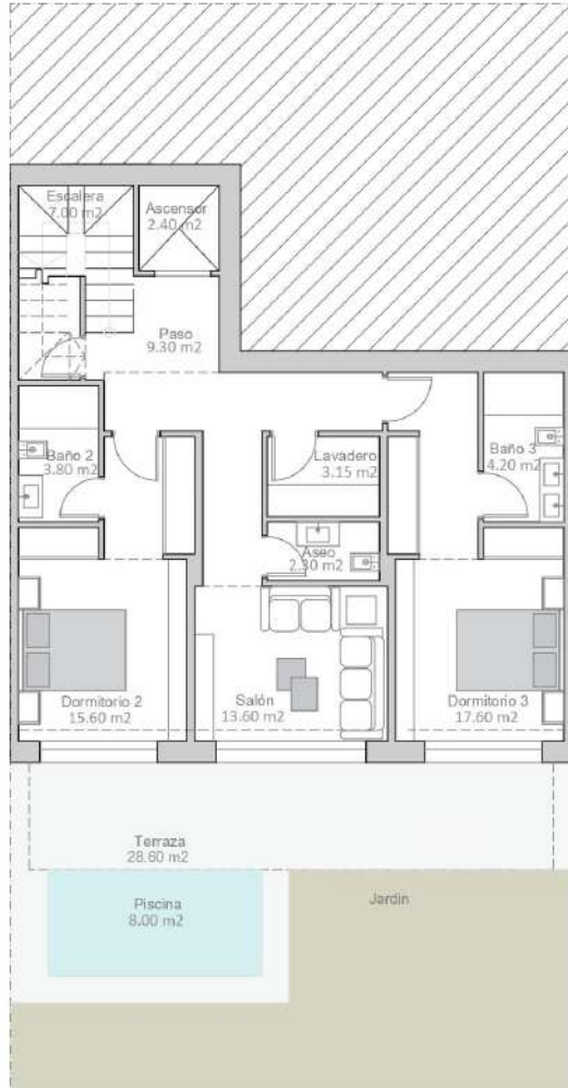
PLANTA BAJA Ground floor
